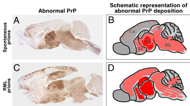
Fig. 2. Histopathologic findings in brains of tga20 mice inoculated with “spontaneous” or brain-derived RML prions. Prions derived from cell cultures exposed to metal wire coated with normal mouse brain homogenate produce a distinctive pattern of PrP deposition in the brain of inoculated tga20 mice. (A) Spontaneously generated prions cause deposition of abnormal PrP in thalamus, brainstem, and, to a lesser extent, superficial layers of the frontal cortex, whereas the hippocampus is strikingly spared. (C) Mouse-passaged RML prions cause a more intense deposition in the superficial layers of the cortex and of the thalamus, and most prominently includes the hippocampus, a feature not seen in any mice inoculated with spontaneous cell-passaged prions. (B and D) Schematic representations of abnormal PrP immunoreactivity. [Scale bar (A and C): 3.5 mm.]
